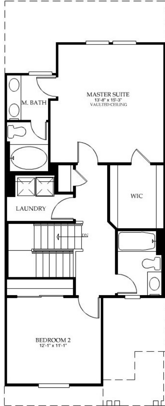
Second Floor
